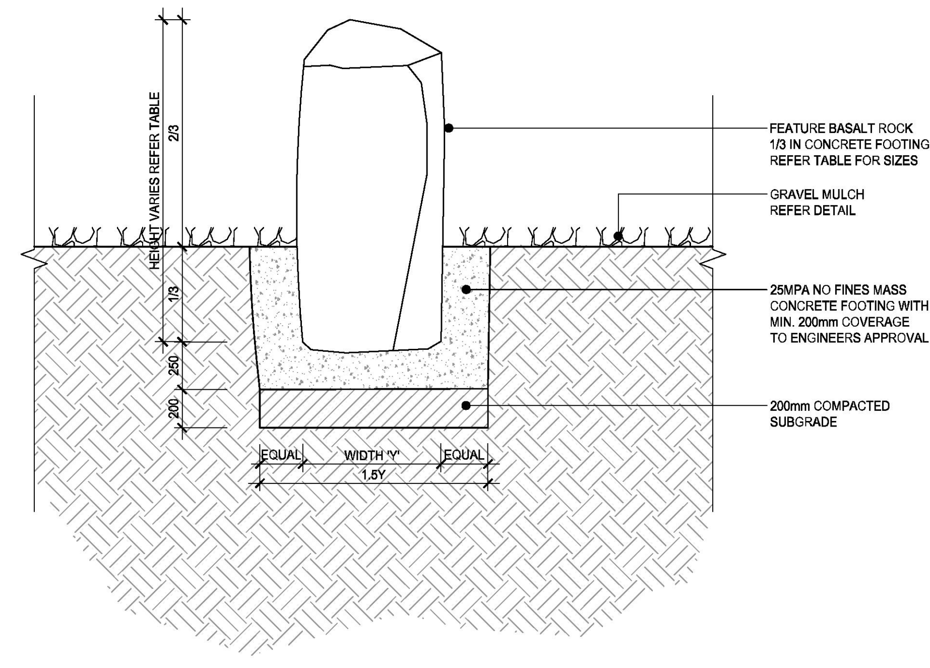
TYPICAL FEATURE ROCK DETAIL
