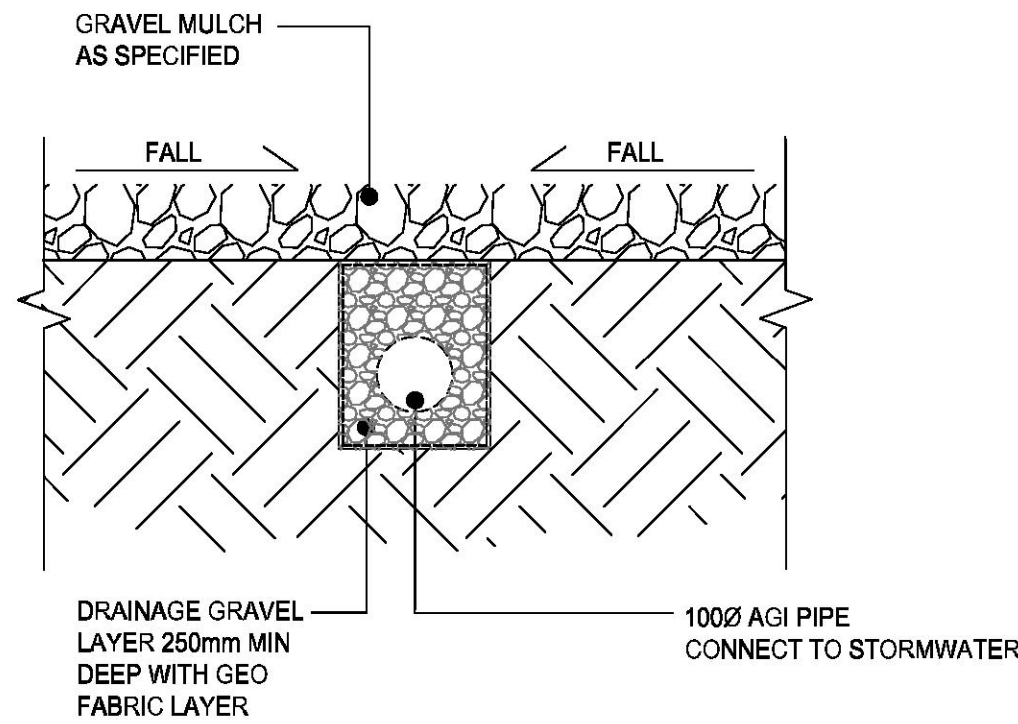
SUB SURFACE DRAINAGE DETAIL
