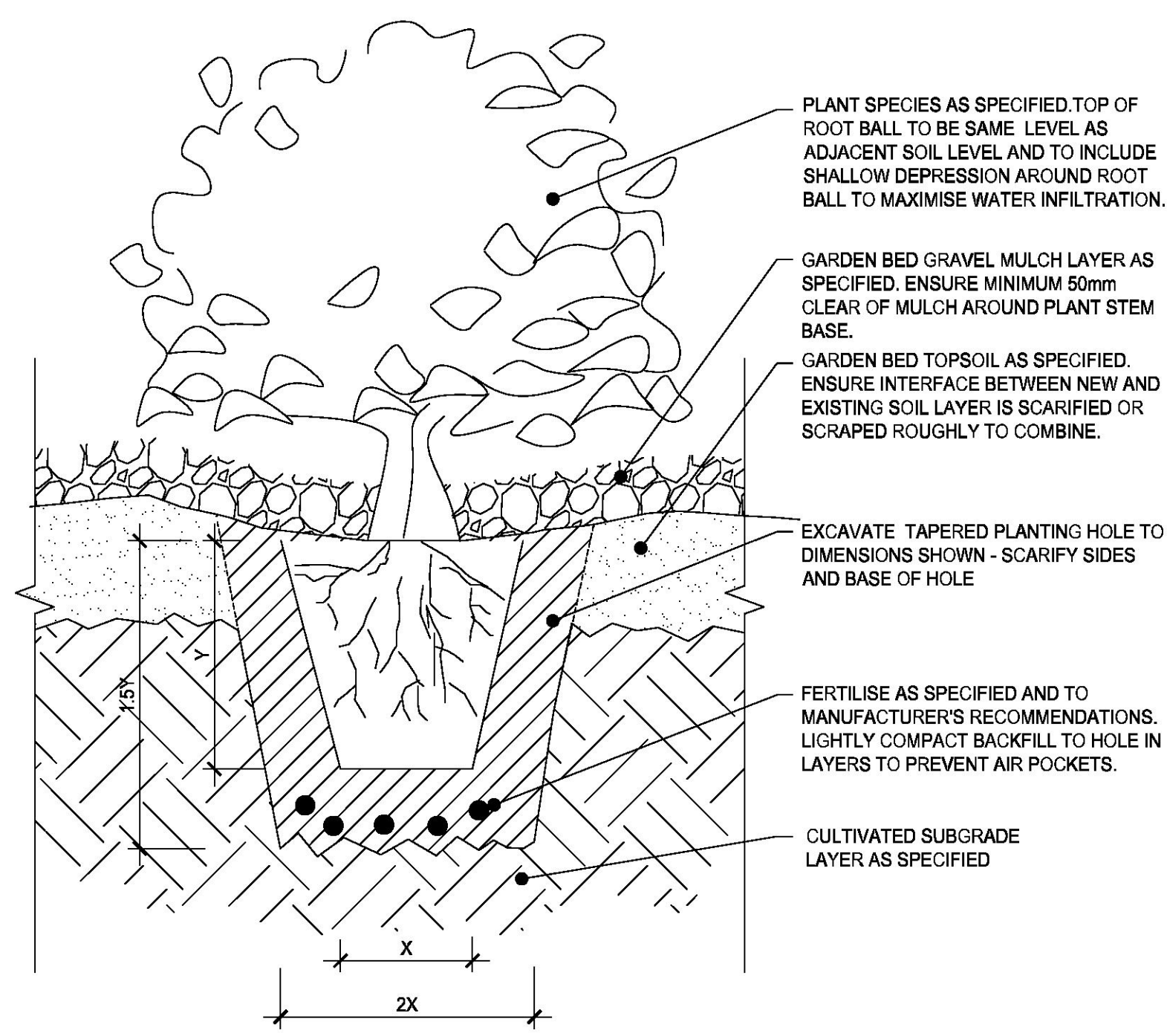
TYPICAL PLANTING DETAIL
