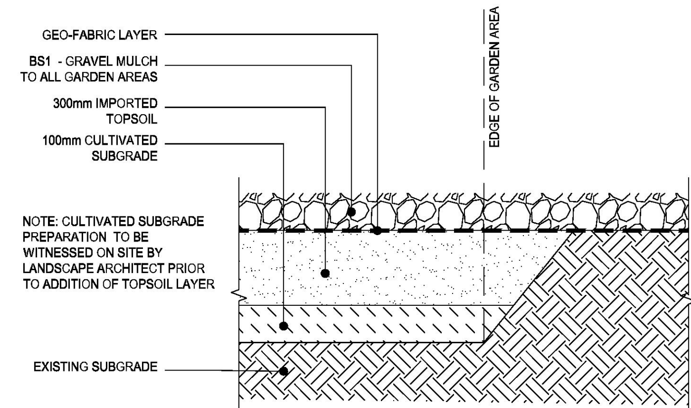
TYPICAL GARDEN AREA
