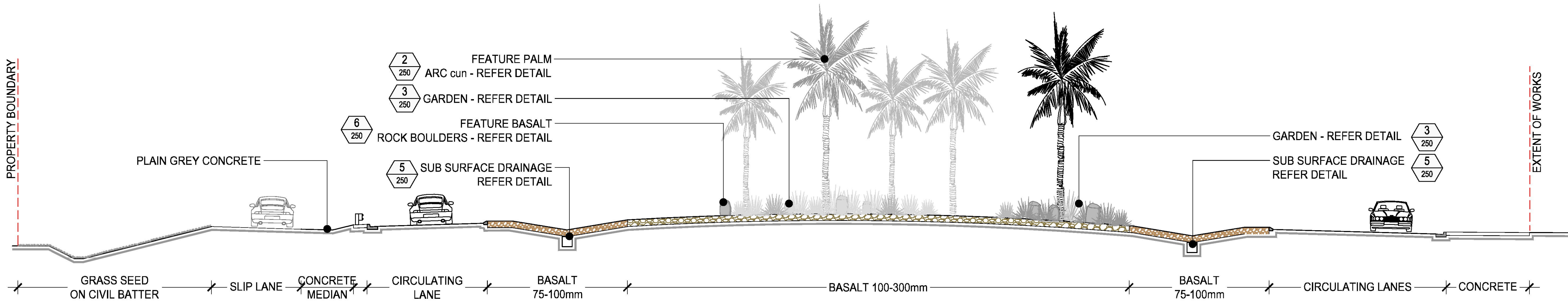
LANDSCAPE SECTION NTS 1 240
